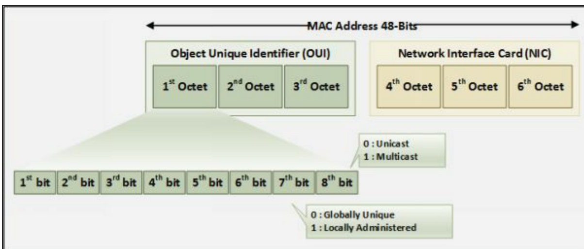
Figure 8-04 MAC-Address
