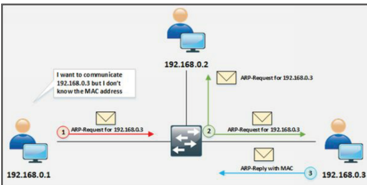
Figure 8-10 ARP Operation
