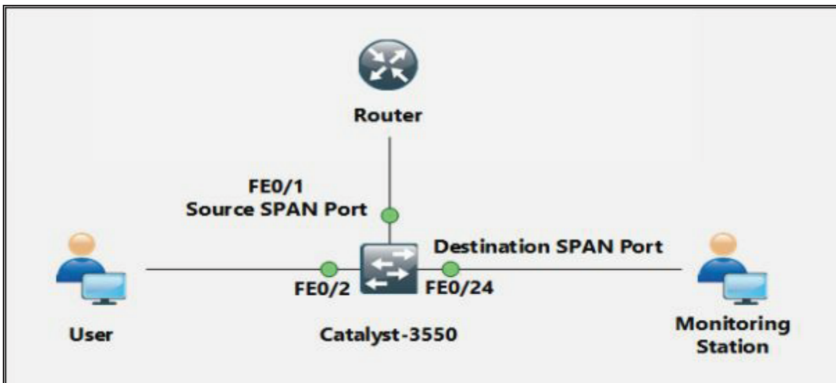
Figure 8-03 SPAN Port
