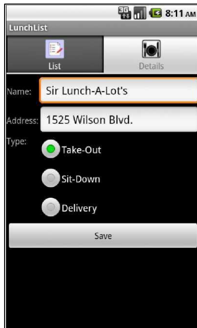
Figure 14. The second tab of the two-tab LunchList
