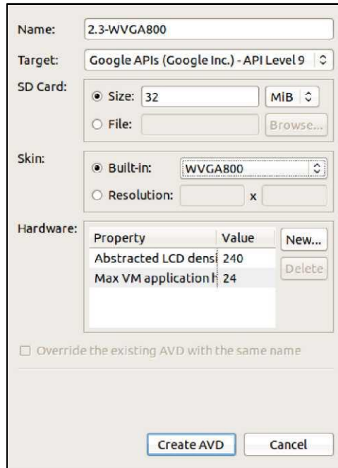
Figure 58. Adding a New AVD (continued)
