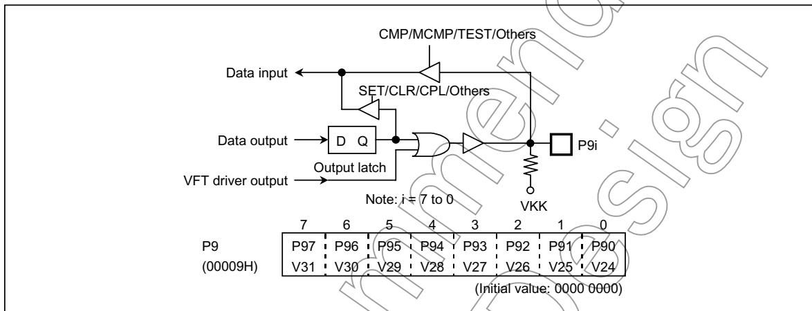
Figure 2.2.11 Port P9
