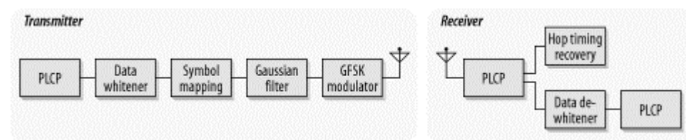
Figure 10-10. Frequency-hopping transceiver
