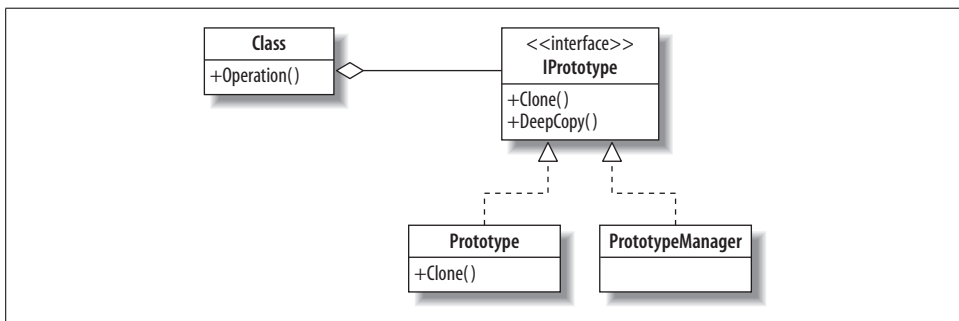
Figure 5-1. Prototype pattern UML diagram
