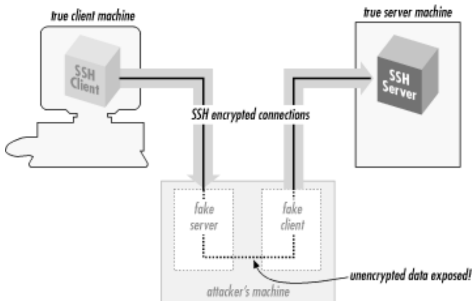
Figure 3.8. Man-in-the-middle attack
