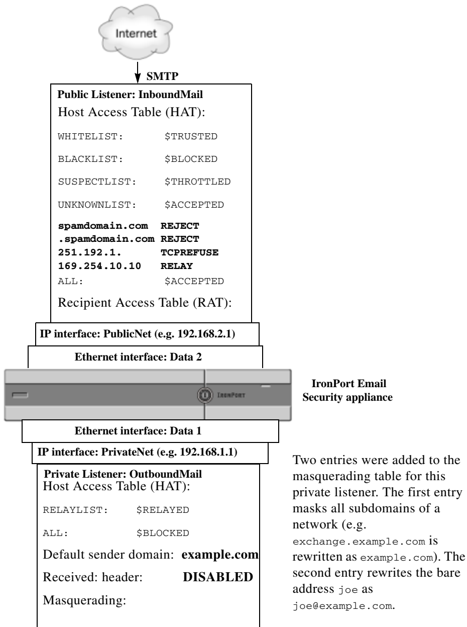
Figure 24-3 Masquerading Defined for a Private Listener
