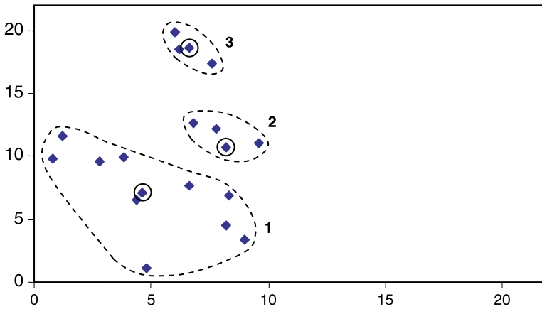
Figure 19.11 Revised Clusters
