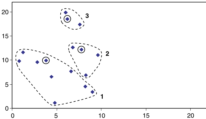
Figure 19.9 Initial Clusters
