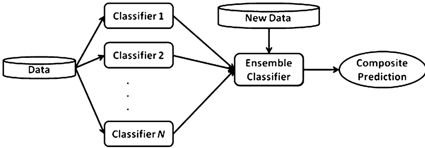
Figure 14.1 Ensemble Classification
